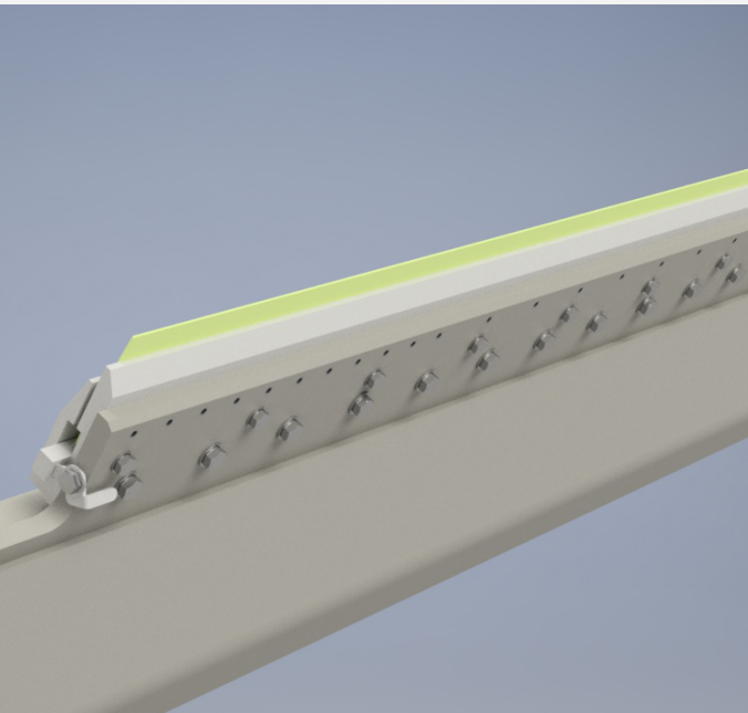
PCut - Yankee doctoring system
